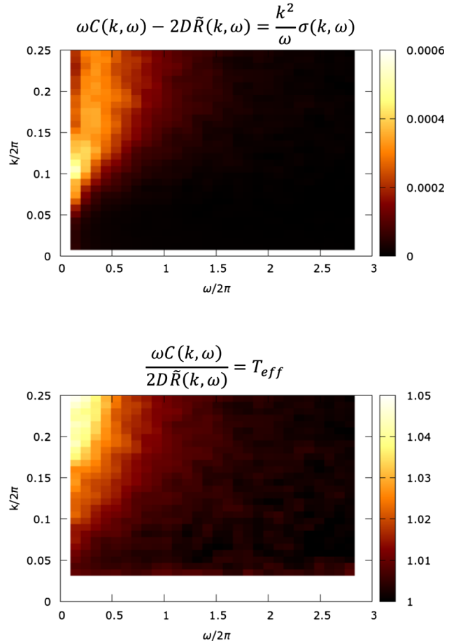
FIG. 5. (a) Correlator-response mismatch \omega C - 2D\dot{R} \propto \sigma_\phi(\mathbf{k}, \omega)k^2/\omega and (b) normalized effective temperature \mathcal{D}(\mathbf{k}, \omega)/D as a function of \mathbf{k} and \omega for Active Model B in one dimension. Parameter values as in Fig. 4. (Control simulations for the passive limit \lambda = 0 recover a statistically insignificant signal for both plots, not shown, confirming that our numerical algorithm respects TRS when present.)
